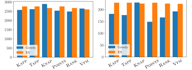
Figure 7: Average social welfare (across elections) using the POINTS- (left) and KNAP-voters (right) to compute welfare.
