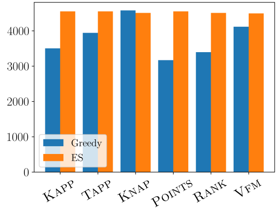
(d) Average social welfare (averaged across elections) using VFM-voters to compute welfare.
