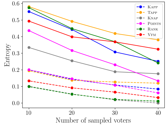
(d) Greedy (full lines) and ES(dotted lines) entropy for each input format (sample format get same color) given different sample size in project set LARGE-B
