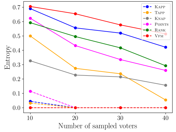
(b) Greedy (full lines) and ES(dotted lines) entropy for each input format (sample format get same color) given different sample size in project set SMALL-B
